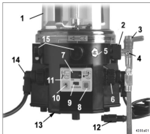
Fig. 2 - Components of pump 233
